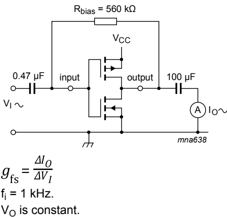
Fig. 10. Test set-up for measuring forward transconductance
