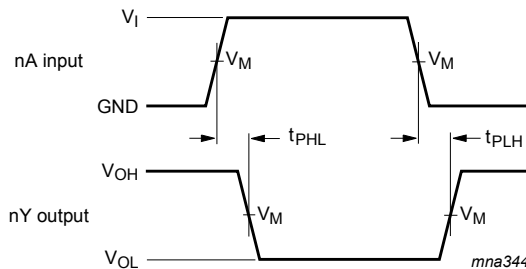
Fig. 7. The input (nA) to output (nY) propagation delay times
